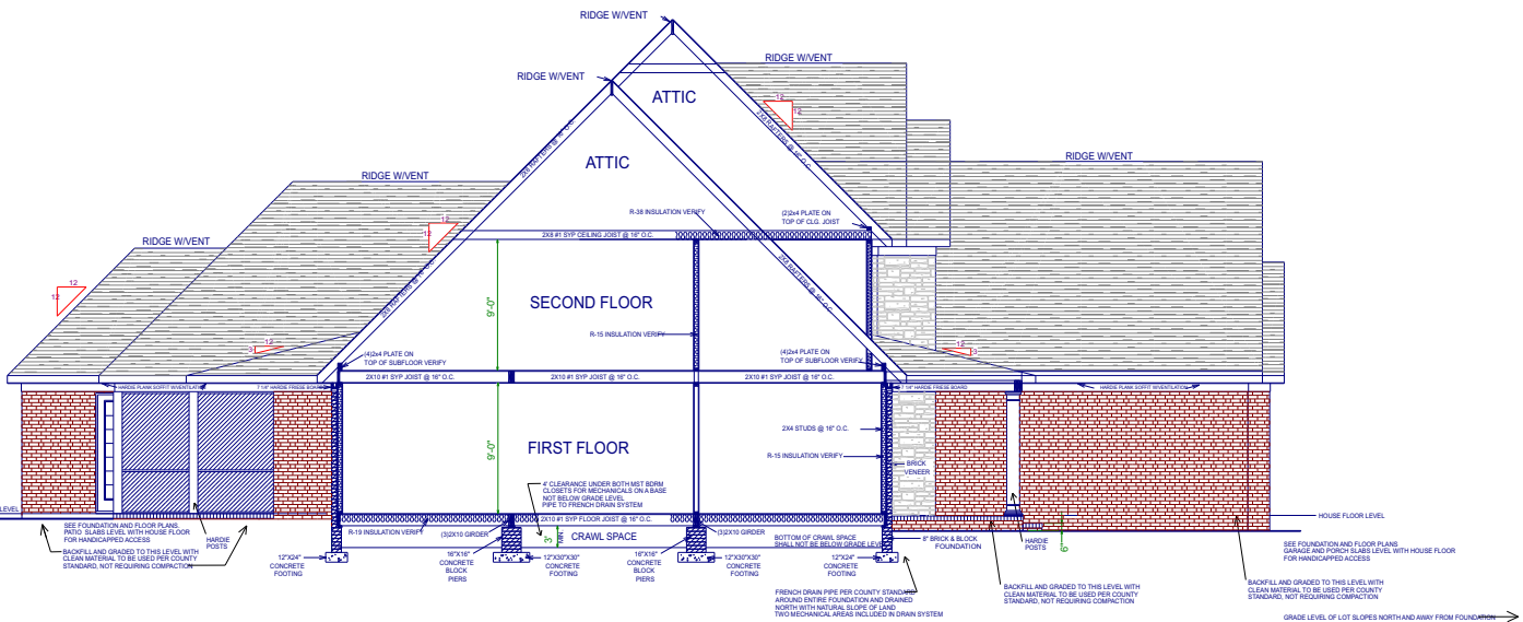
SECTIONAL DETAIL SCALE-1/4"=1'-0"
